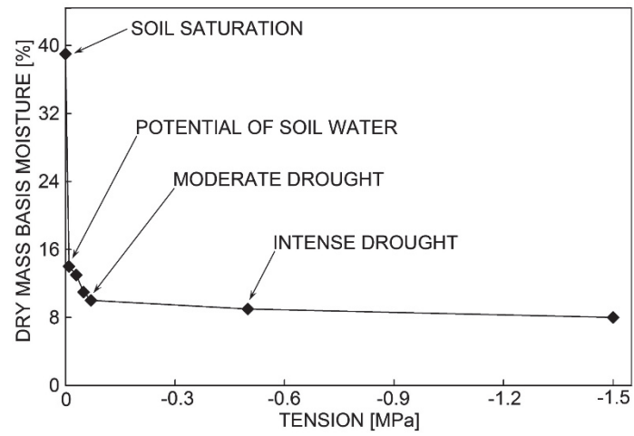
Fig. 1 Suppl. A water retention curve of the soil (the Richards pressure plate) used to define water management.
