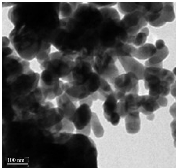
Fig. 1. Suppl. Morphological characterization of copper oxide nanoparticles in a \frac{1}{2} MS liquid medium using transmission electron microscopy (the scale bar represents 100 nm).
