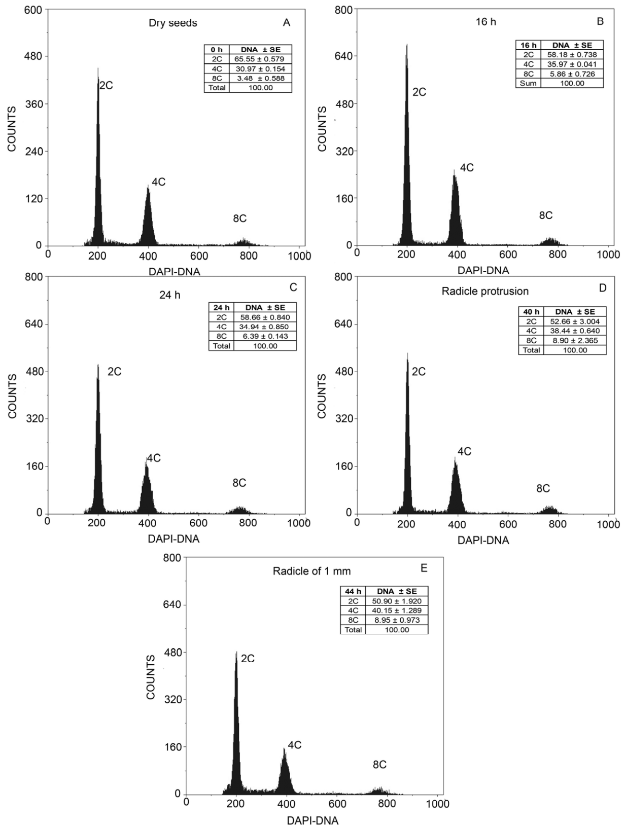
Fig. 1 Suppl. Flow cytometry profiles of Leucaena radicles excised from seeds at different stages during germination. Radicles were excised from dry seeds (A), 16 h imbibed seeds (B), 24 h imbibed seeds (C), seeds at the point of radicle protrusion (D), and seeds with a radicle length of 1 mm (E).
