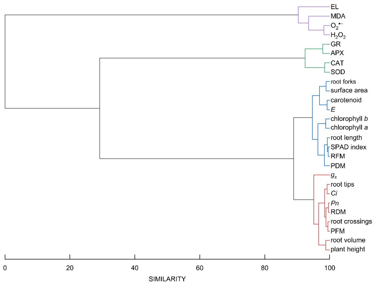
Fig. 1 Suppl. A dendrogram of hierarchical cluster analysis (complete clustering algorithm) indicating similarities and dissimilarities among various plant characteristics under salinity stress.
