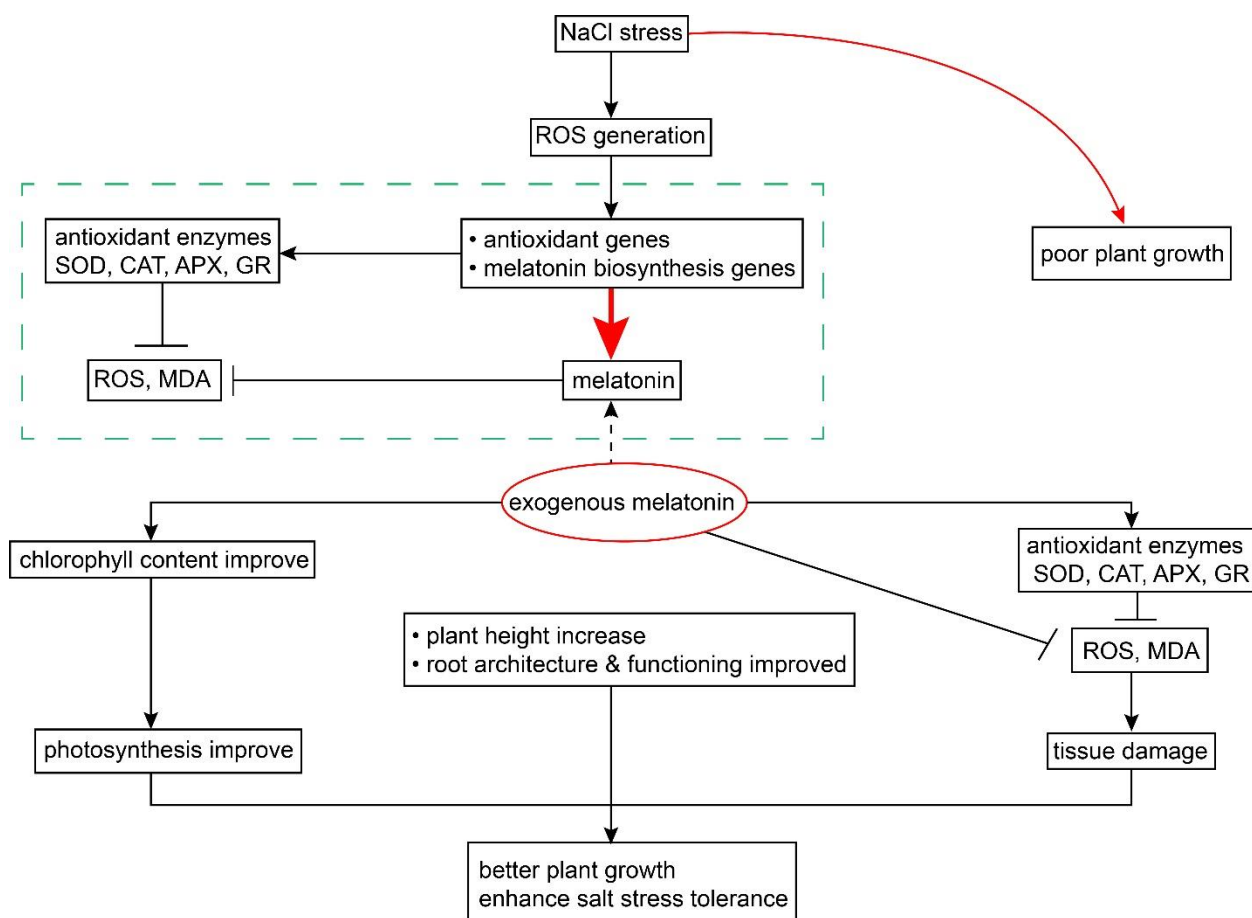
Fig. 2 Suppl. A schematic diagram showing NaCl stress tolerance in tomato seedlings pretreated with melatonin. As the concentration of melatonin was not measured exactly in the study, a phenomenal expression of melatonin biosynthesis genes is represented by red bold arrows .
