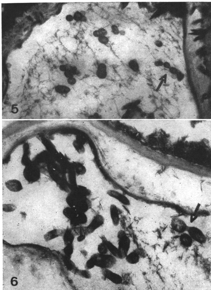
Fig. 5. A chain of dense coccoid bodies (arrow) in an abnormal sprout (13 000 \times ).
