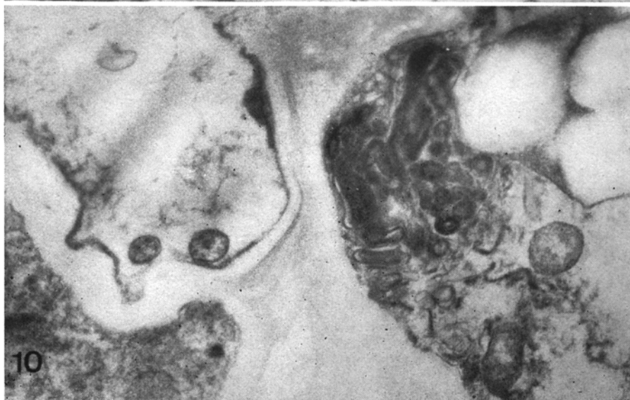
Fig. 9. Mycoplasmas in an abnormal sprout. Note internal structures, constrictions, and denser ends of some filaments (39 000 \times ).
