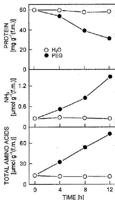
Fig. 3. The contents of protein, ammonia, and total amino acids in detached rice leaves floating on water ( \text{H}_2\text{O} ) or PEG (-1.5 MPa) solution for 4, 8, and 12 h. Means \pm SE, n = 4 .
