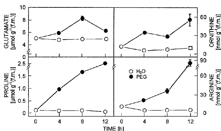
Fig. 2. The contents of proline, glutamic acid, arginine, and ornithine in detached rice leaves floating on water ( \text{H}_2\text{O} ) or PEG (-1.5 MPa) solution for 4, 8, and 12 h. Means \pm SE, n = 4 .
