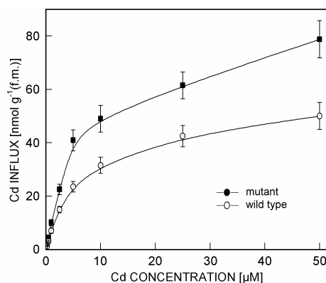
Fig. 3. Concentration-dependent \text{Cd}^{2+} uptake in roots of intact mutant and wild type rice seedlings. Means \pm SE of four replicates.
