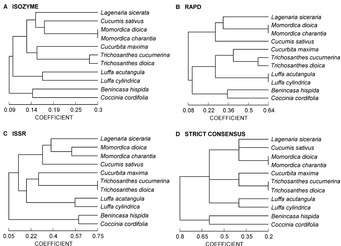
Fig. 2. Dendrograms generated using unweighted pair group method with arithmetic average (UPGMA) analysis, showing relationships between different members of Cucurbitaceae , using isozyme (A), RAPD (B), ISSR (C) data and a strict consensus tree based on both RAPD and ISSR data (D).
