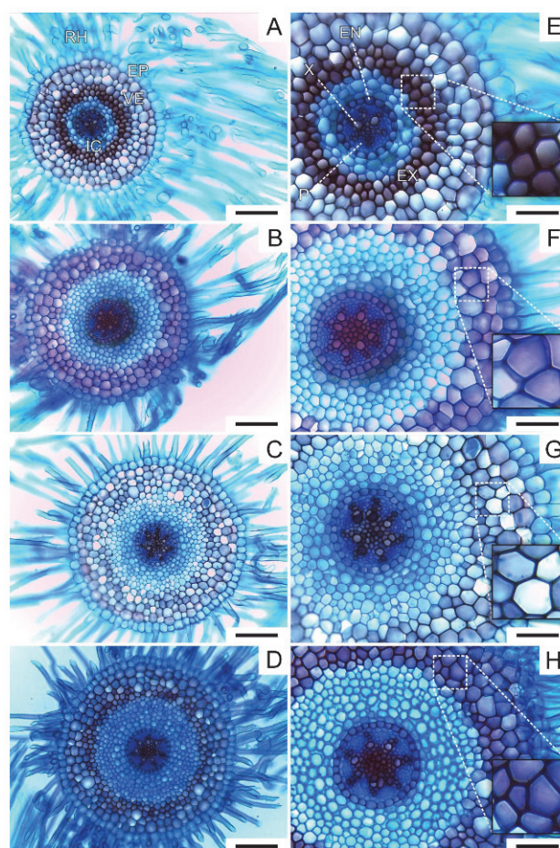
Fig. 2. Root cross sections of Aechmea blanchetiana plantlets grown on a medium with different NAA concentrations: 0 (A,E), 2 (B,F), 4 (C,G), and 6 \mu M (D,H) for 50 d. RH - root hair, EP - epidermis, VE - velamen, IC - inner cortex, EX - exodermis, EN - endodermis, X - xylem, and P - phloem. Bars = 100 \mu m (A-D) and 50 \mu m (E-H).
